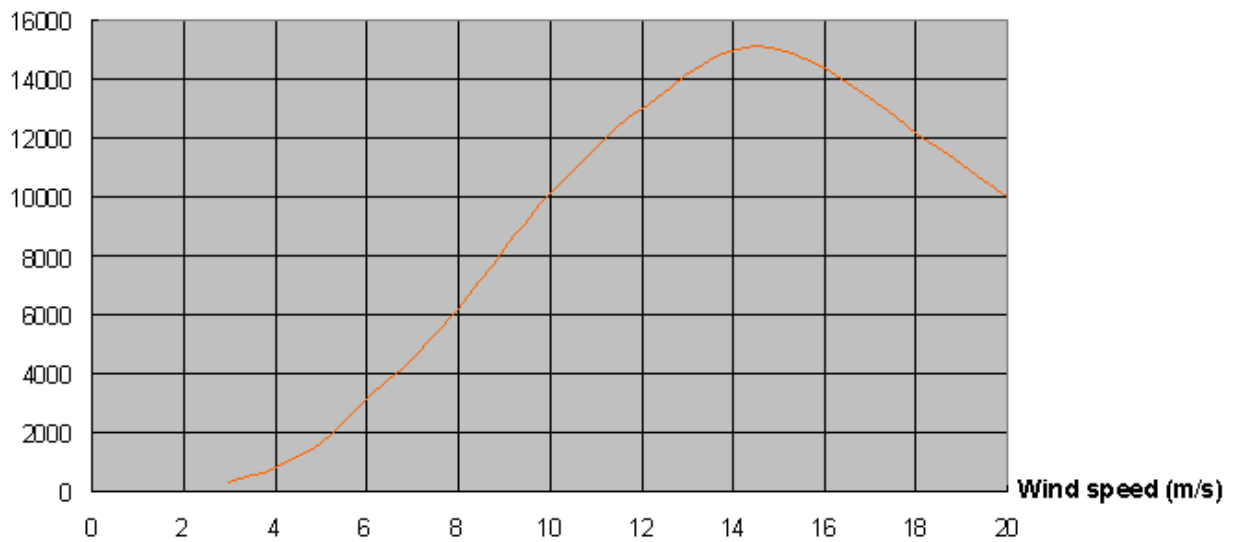
HUMMER-10KW Wind Generator
